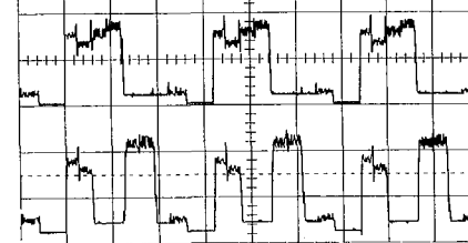
IC201 pin 20 4v4 p.p. at 20 \mu sec
